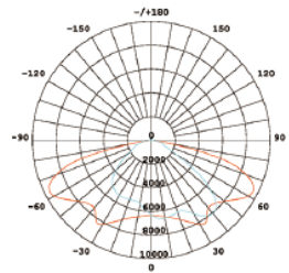
T2S2201 IESNA Type II Short
