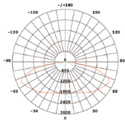
T2S2321 IESNA Type II Short
