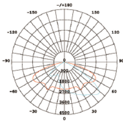
T2S1324 IESNA Type II Short
