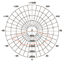
T3M1321 IESNA Type III Medium
